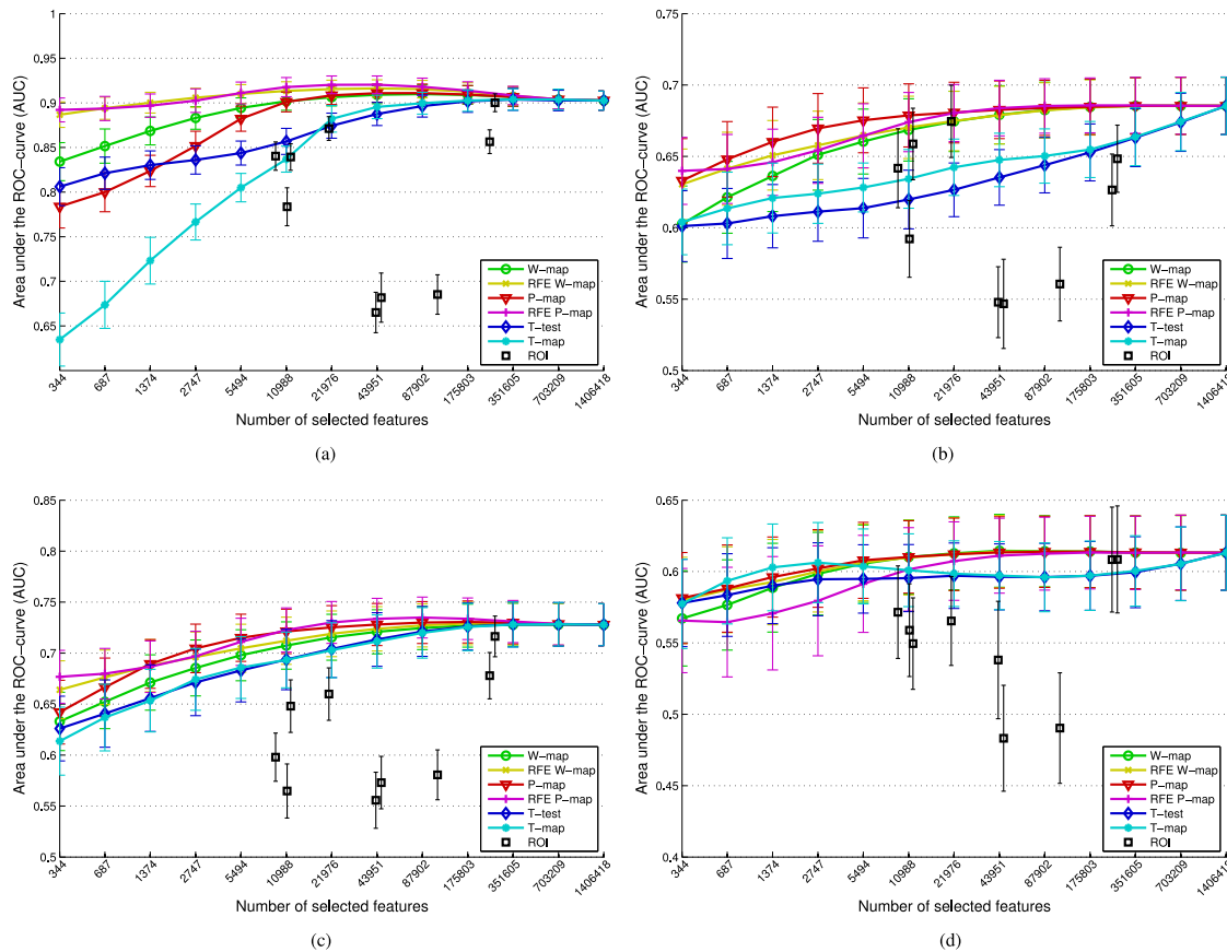
Fig. 2. Classification area under the ROC curve (AUC) as function of number of selected features for seven feature selection methods. The mean and standard deviation of AUC are shown over 100 cross validations for (a) AD-CN, (b) AD-MCI, (c) MCI-CN, and (d) MCIc-MCInc classification.
